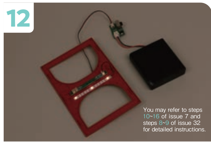
Plug the Connection Cable's connector into the socket on the other side of the Ceiling, connect it to the Battery Box and other parts, and check that the LEDs light up properly.
