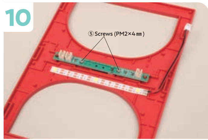
Tighten the ⑤ Screws (PM2×4mm) into the two holes in the Circuit Board as shown.
